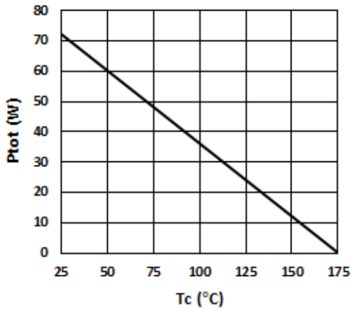
Fig 7 Power Derating
